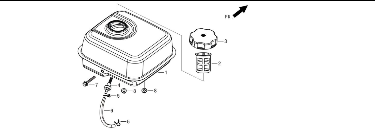
FIG.12 TANK ASSY, FUEL (F01)
