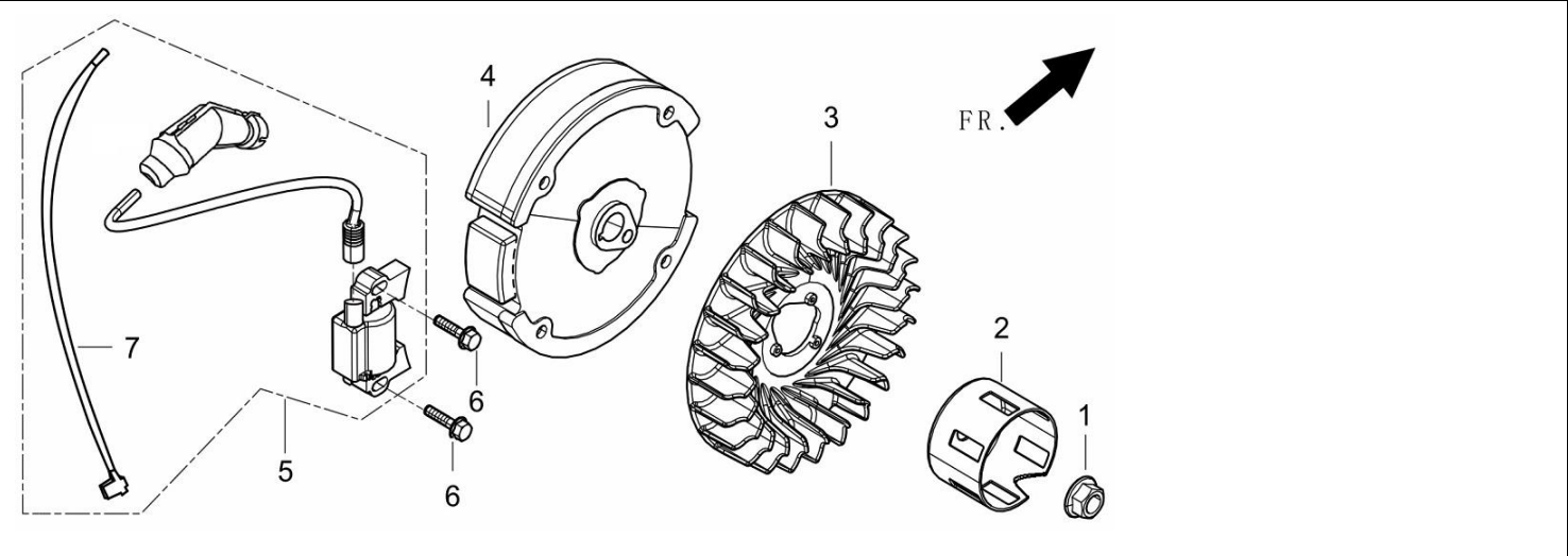
FIG.13 FLYWHEEL / IMPELLER / STARTER PULLEY / IGNITION COIL (E15)
